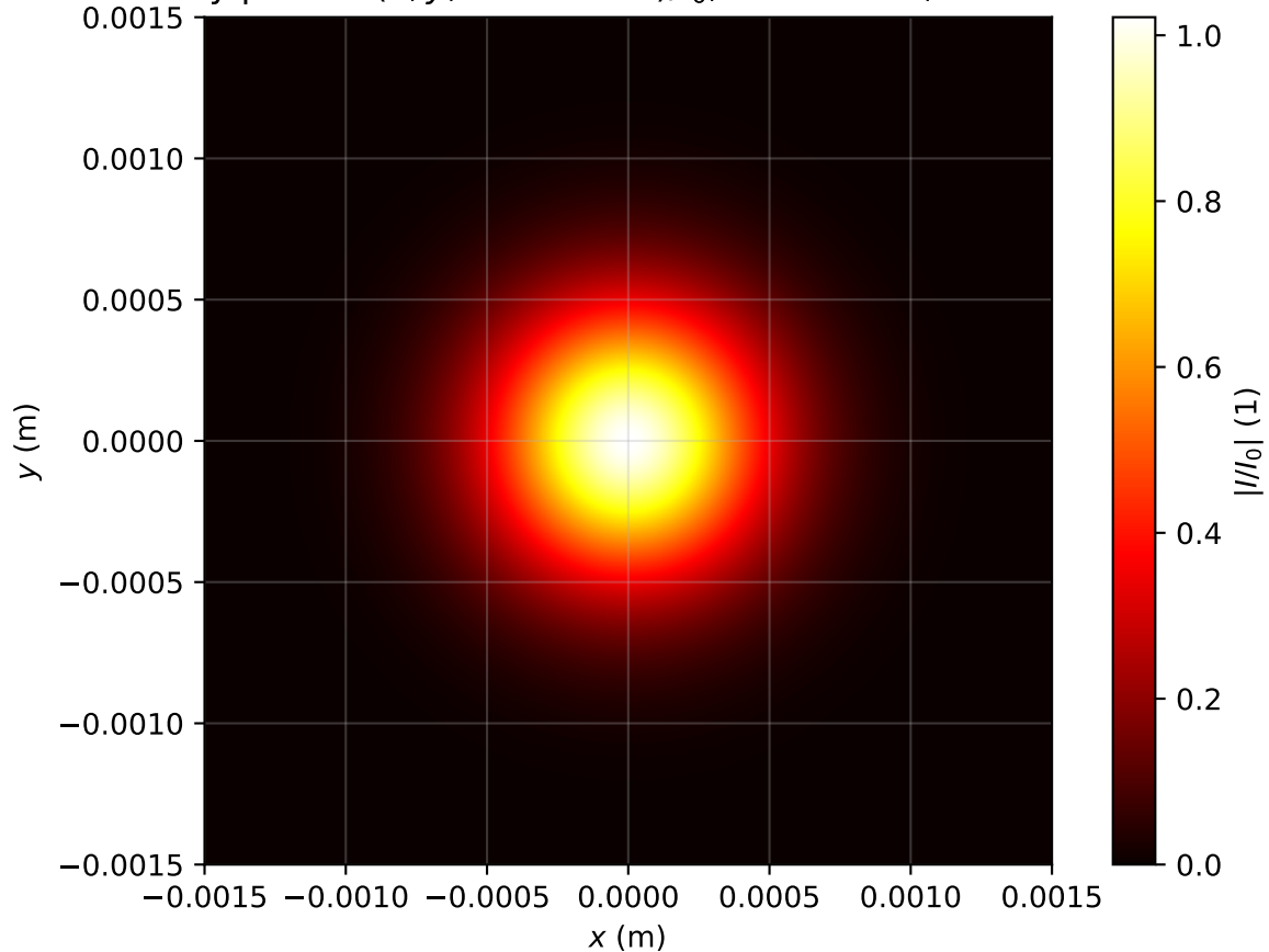
Intensity profile I(x, y, z = 0.557m)/I_0 , Pin=0.4Pcr, artificial time
